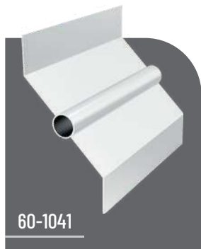
60-1041 Z-TYP ZAUNPROFIL Z TYPE FENCE PROFILE
